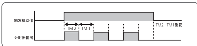
[图29] 计时动作Flicker 2
