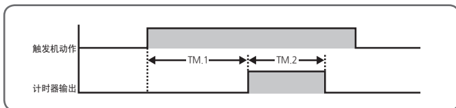
[图27] 计时动作Delay 2
