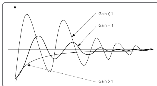
[图5] 演算增益(AT GAIN)
