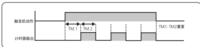
[图28] 计时动作Flicker 1
